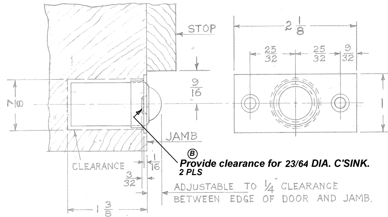
346 CATCH MOUNTED IN JAMB
