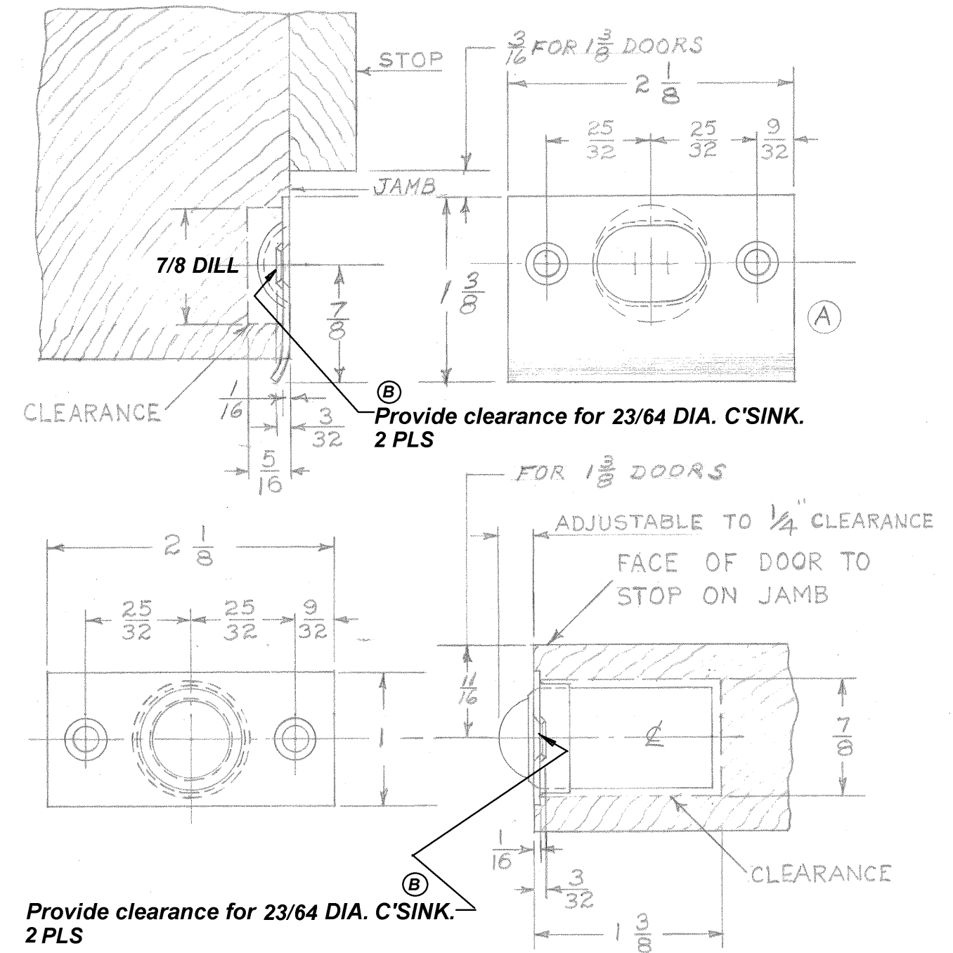
347 CATCH MOUNTED IN DOOR
